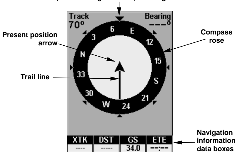
Navigation Page, recording a trail, traveling east. Page looks like this when iFINDER is not navigating to a waypoint, following a route, or backtracking a trail.
